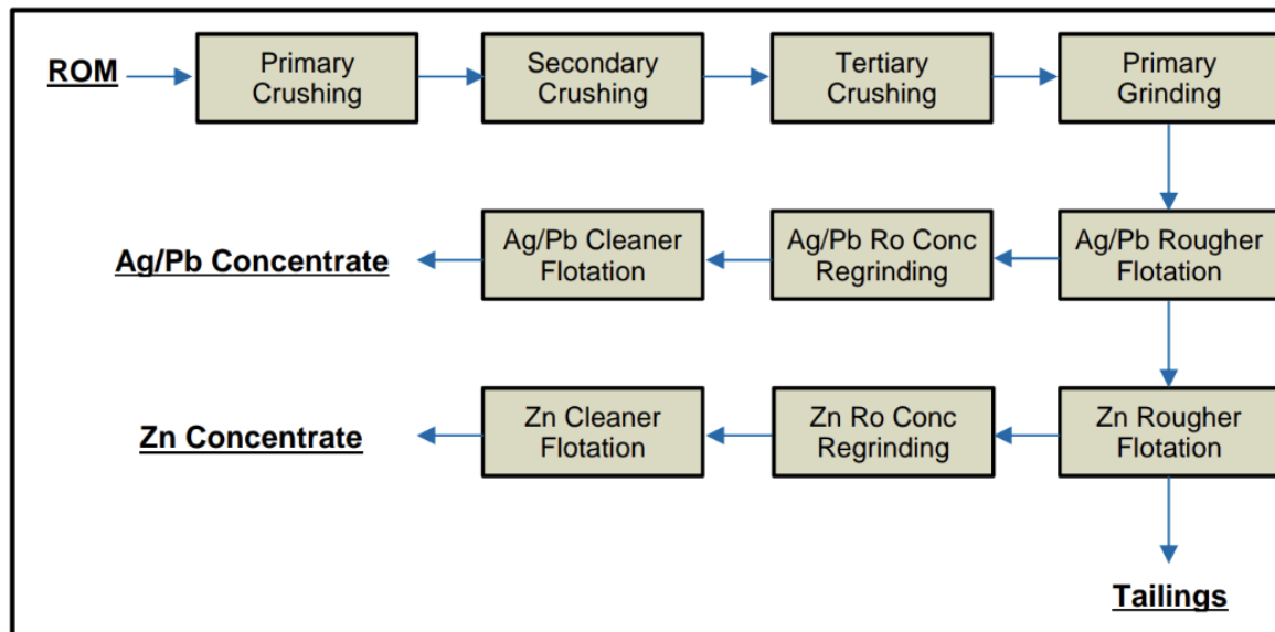
Figure 14-1: Chinchillas Processing Flowsheet Overview
