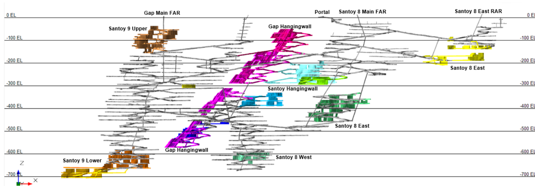
Figure 13-1: Santoy Mine Long Section Looking North
