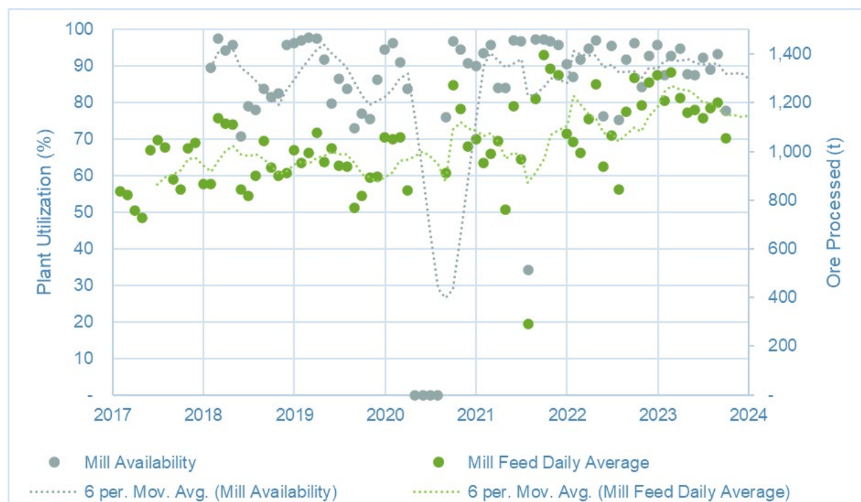
Figure 10-3: Plant Average Daily Throughput and Utilization
