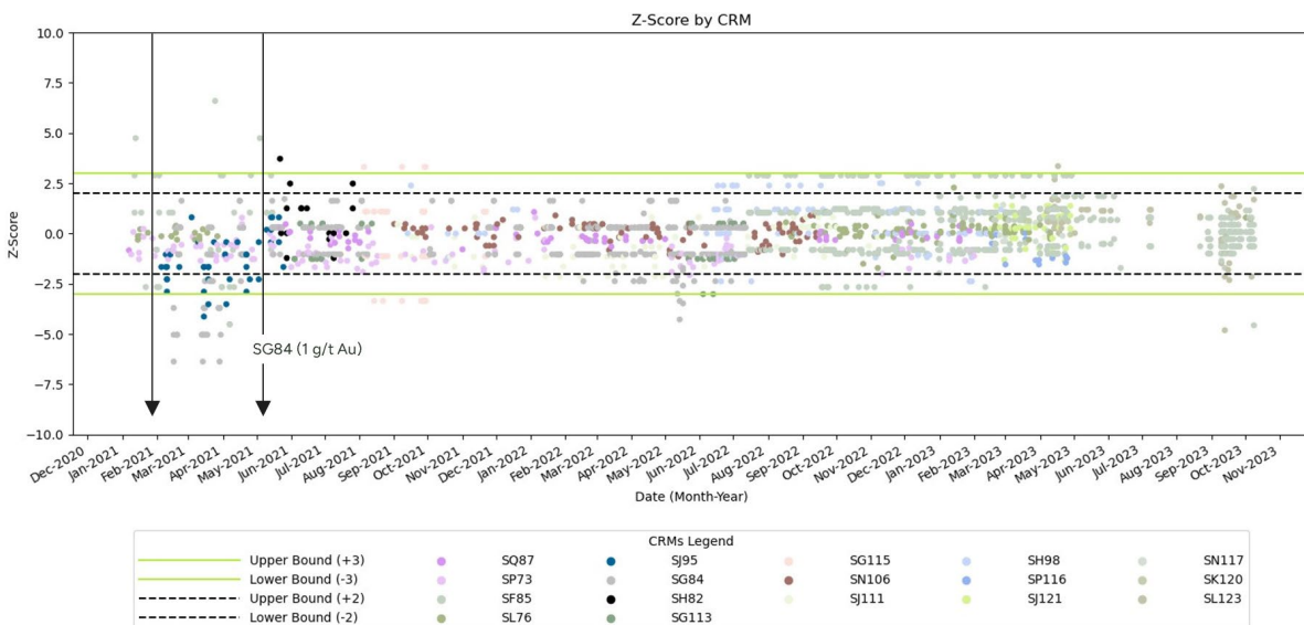
Figure 8-1: Z-score Scatter Plot
